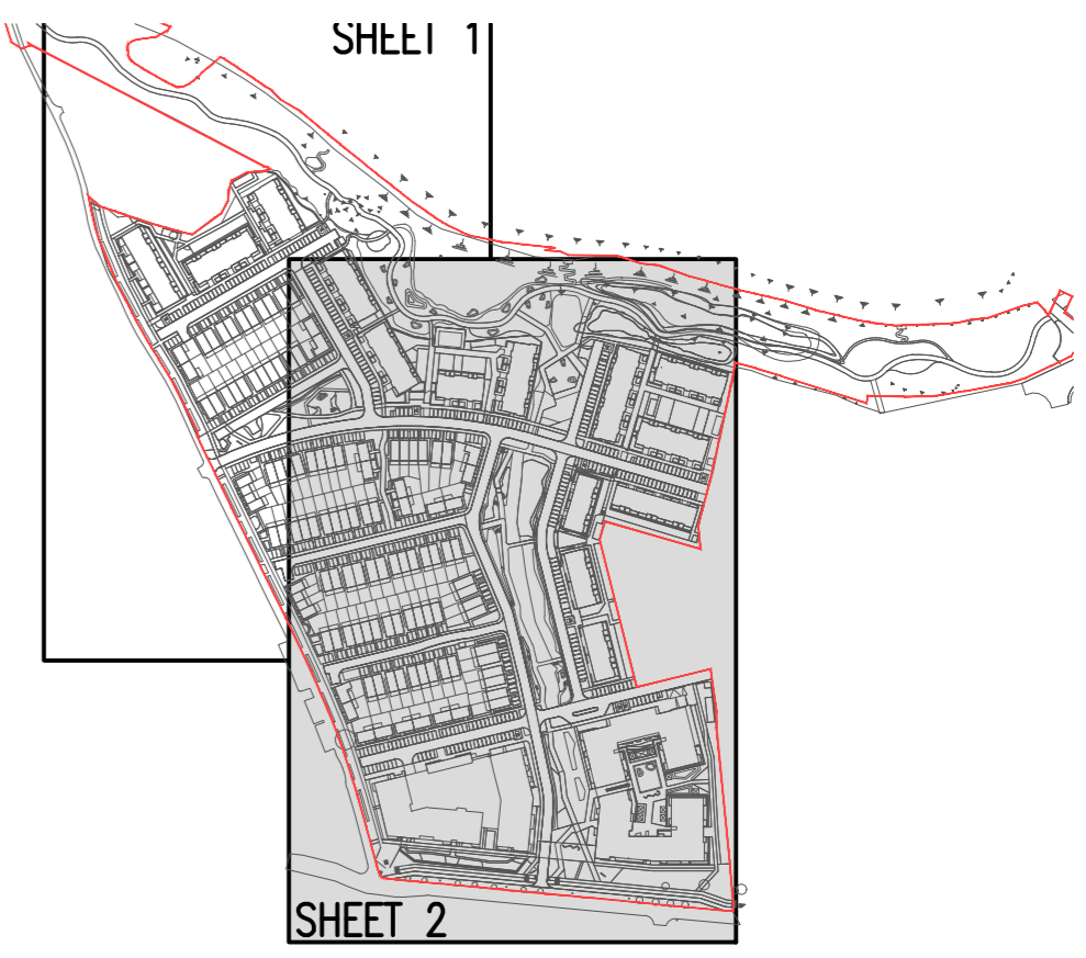
KEYPLAN SCALE 1:5000
